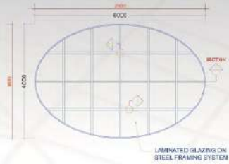
1 TYPICAL PLAN OF WALKABLE SCALE: 1:100
