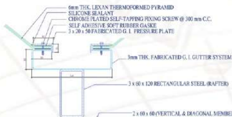
SEC. DET. "T2" A-12 DIM. IN mm NTS
