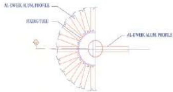
SEC. DET. "L2" A13 DWA 10 mm NTS
